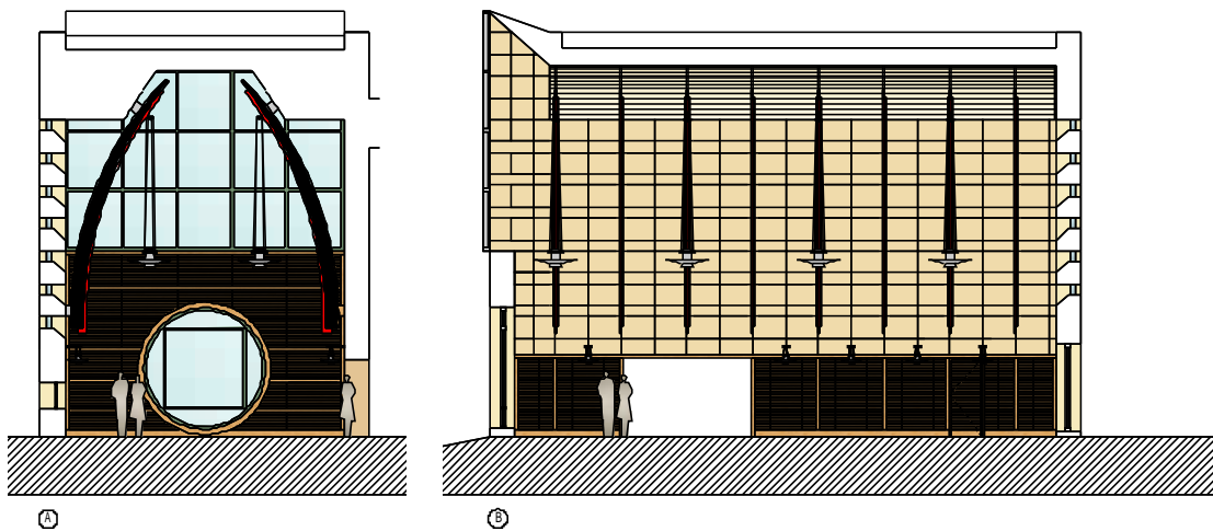
1 ROOM 119-G: DINNING PAVILION INTERIOR ELEVATIONS 3/4"=1'-0"
