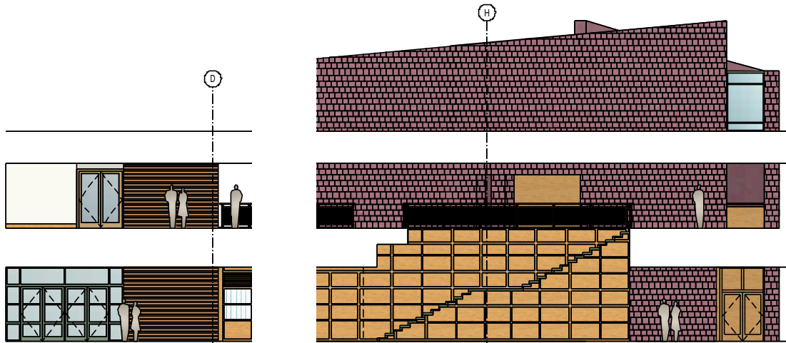
3 ROOMS 100, 200: 1ST FLOOR LOBBY AND 2ND FLOOR CIRCULATION INTERIOR ELEVATION A.8114.3 1/4"=1'-0"
