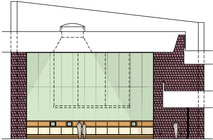
3 ROOM 108: FIREPLACE LOUNGE NORTH SHELL WALL UNFOLDED ELEVATION 18'x11'-0"
