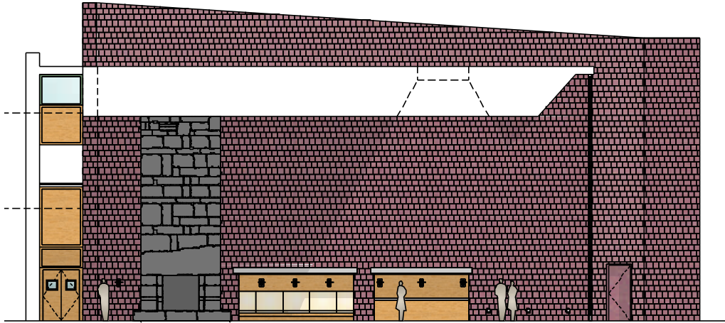
4 ROOM 108: FIREPLACE LOUNGE SOUTH SHELL WALL UNFOLDED ELEVATION 18'x11'-0"
